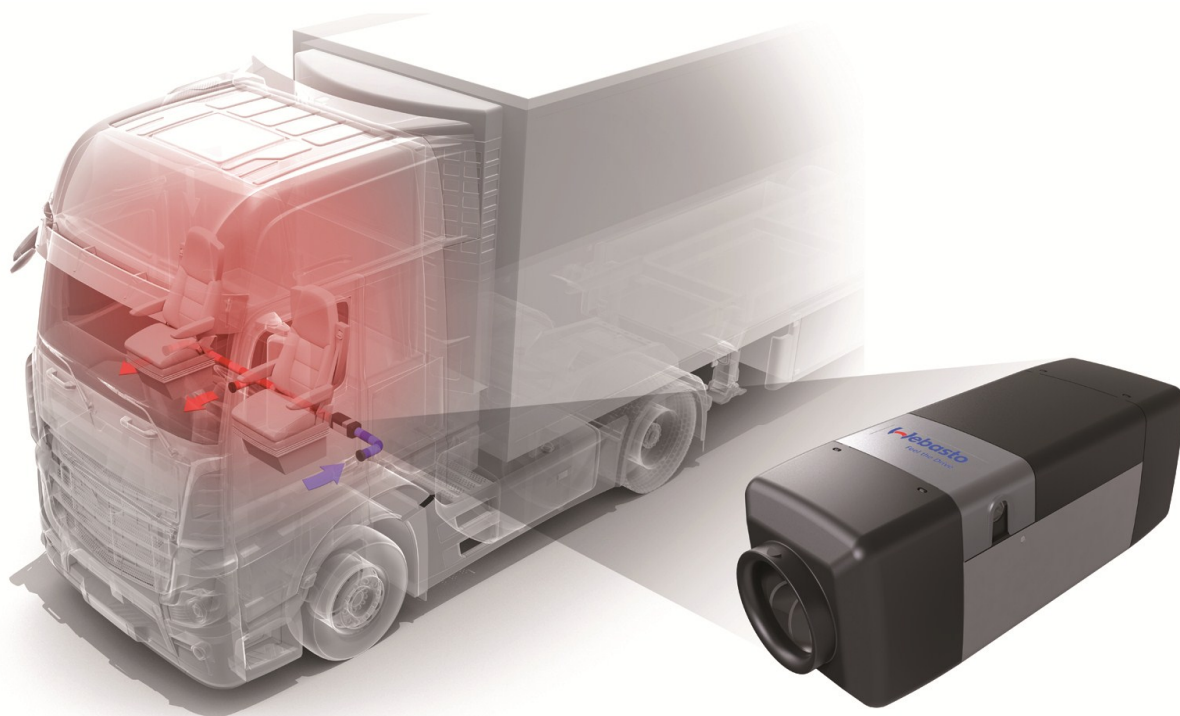
Sample Installation for the Webasto Air Top 2000ST
